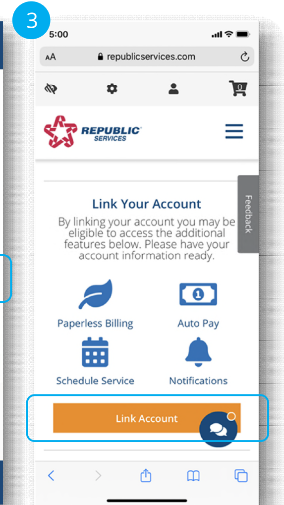
(Web browser)
