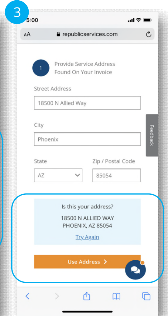
(Web browser)
