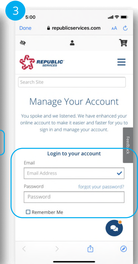
(Web browser)
